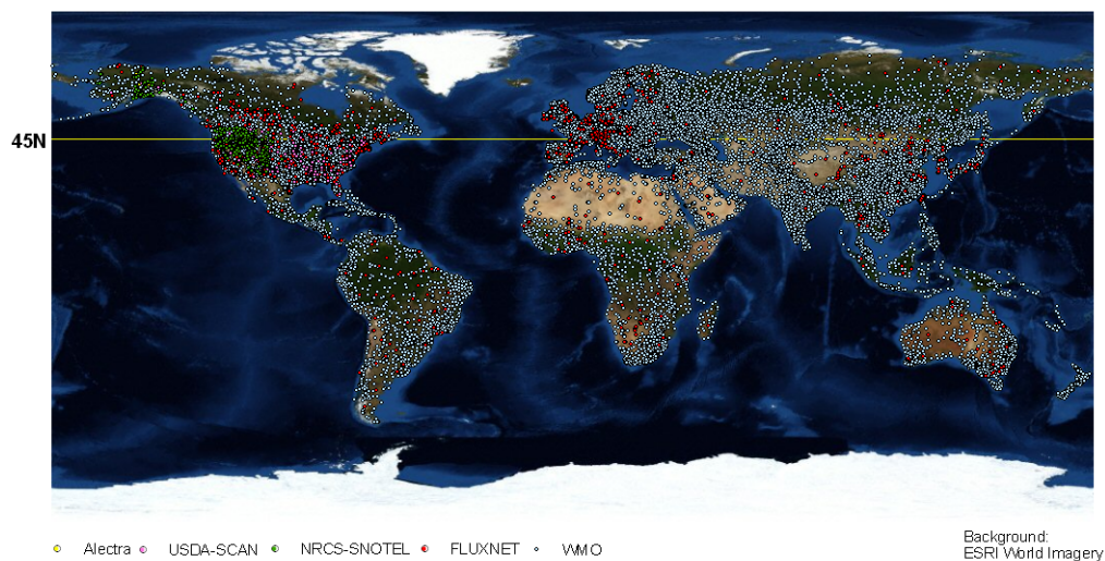
Figure 3-2. World Meteorological Organization's (WMO) global meteorological observation station network (the white dots) with ALECTRA, USDA-SCAN, NRCS-SNOTEL, FLUXNET networks (see Table 3-1). Note that the WMO sites cannot be used directly for comparison with satellite products since they do not measure soil moisture or freeze/thaw state.
