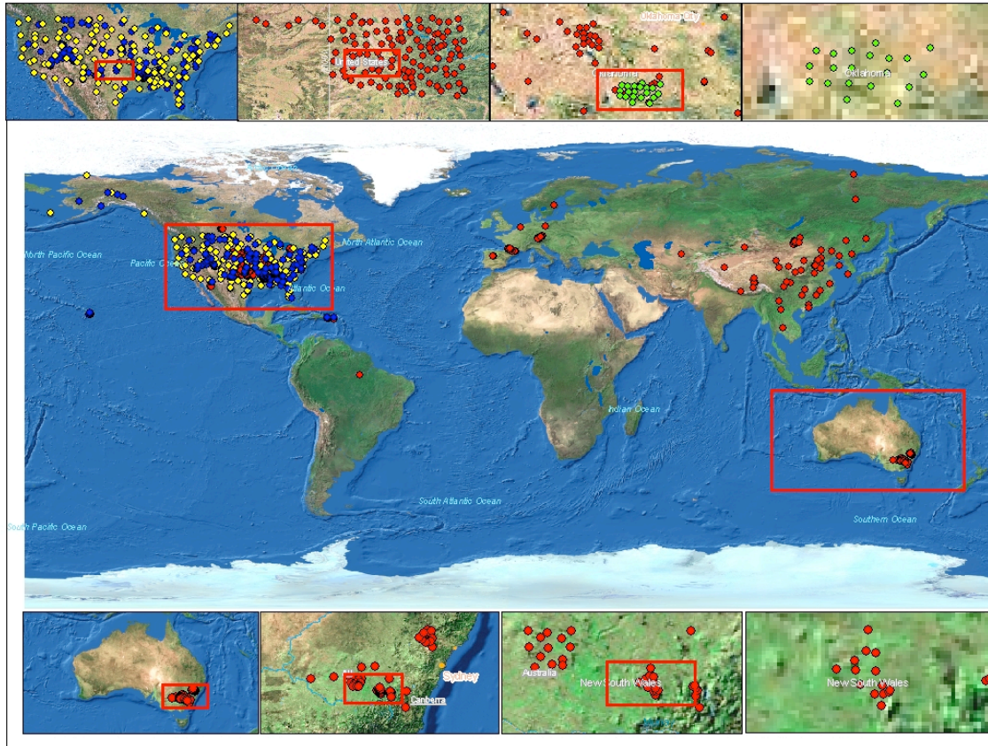
Figure 3-1. In Situ Soil Moisture Resources (v. May 2008). The top panel shows (from left to right) the SCAN and CRN, Oklahoma Mesonet, and Little Washita Networks. The bottom panel shows Australia and a sequence of enlargements to the Kyeamba area.
