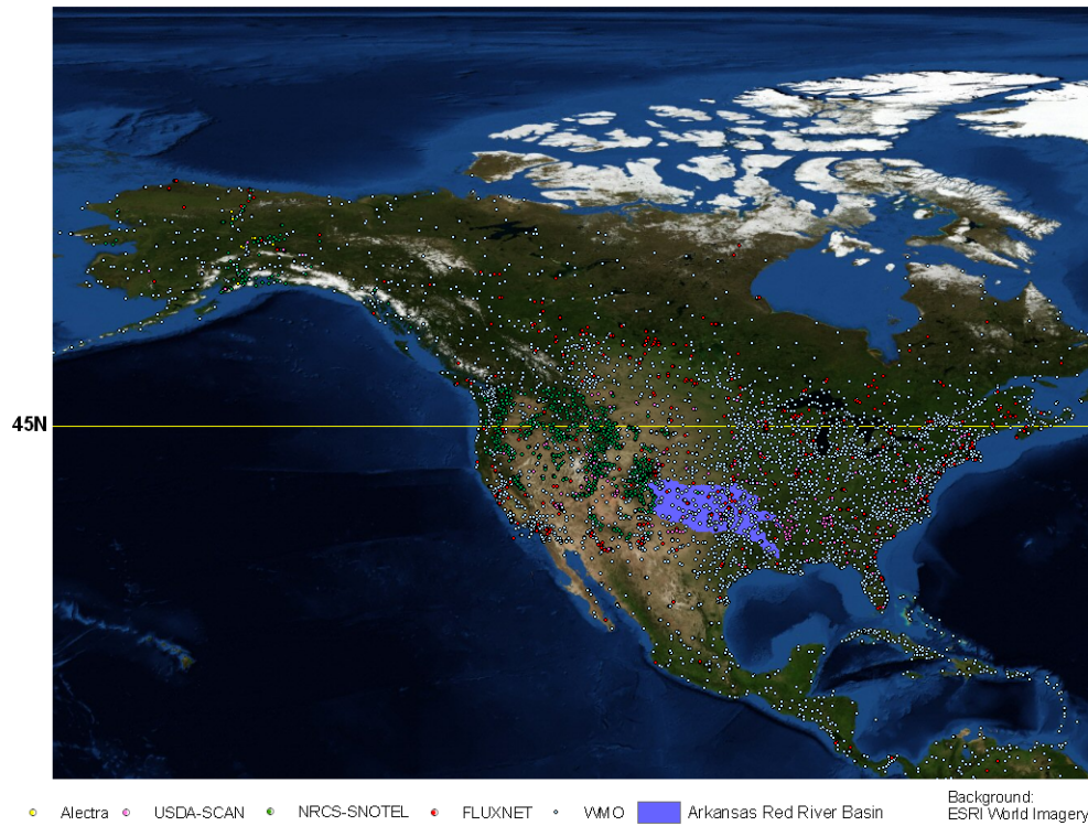
Figure 3-3. WMO's meteorological observation stations in North America (the white dots) with ALECTRA, USDA-SCAN, NRCS-SNOTEL, FLUXNET networks (see Table 3-1). The Arkansas Red River Basin is marked with blue color. The basin contains among others over hundred observation stations by Oklahoma Mesonet. Note that the WMO sites cannot be used directly for comparison with satellite products since they do not measure soil moisture or freeze/thaw state.
