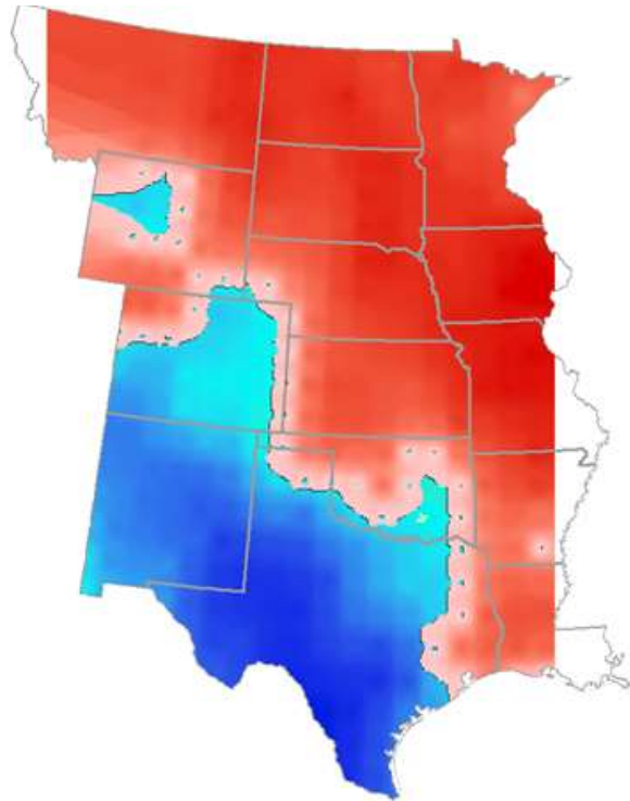
Prediction using Soil Moisture Estimate
