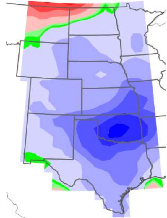
Observed Rainfall Anomalies
